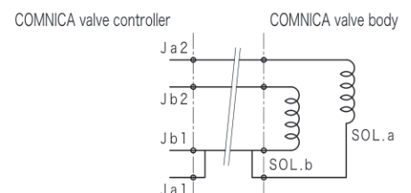
Method of connecting the wires between the controller and valve body
