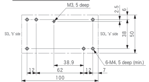
Controller mounting dimensions
